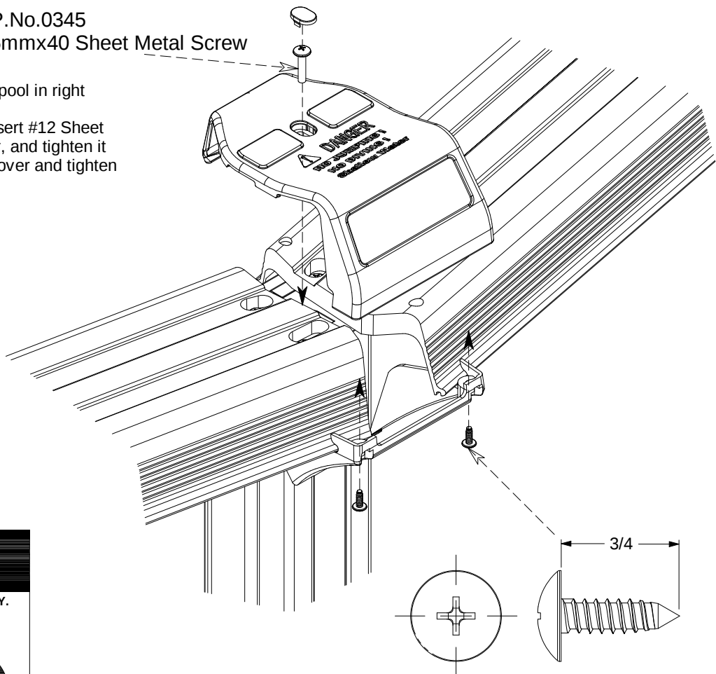
P.No.0341 #12 Sheet Metal Screw
