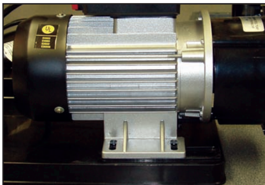
4A— Cradle style mount pump
