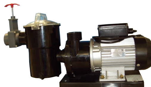
Figure 14 — Pump with slide valve in pump inlet
