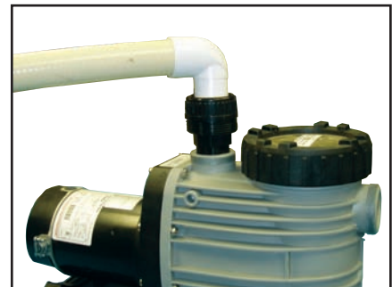
Figure 22 — Attaching flex pipe to pump
