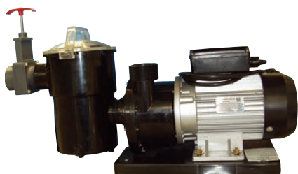
Figure 3b — Pump with slide valve in pump inlet
