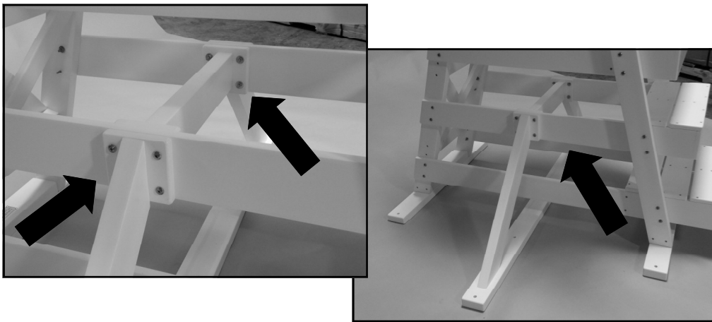
6. Attach center brace to third platform using four 3" bolts for each side.
