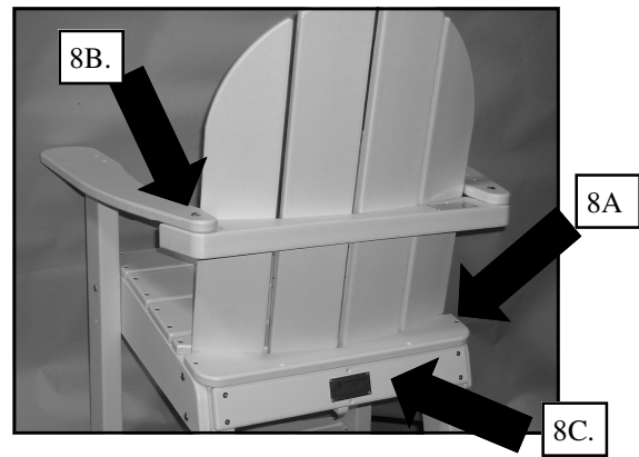
8A. Attach back rest to seat section using four 1 5/8" screws. 8B. Attach back rest to right and left arms using two 2 1/2" bolts. 8C. Attach back leg section to center seat support using two 1 5/8" screws.
