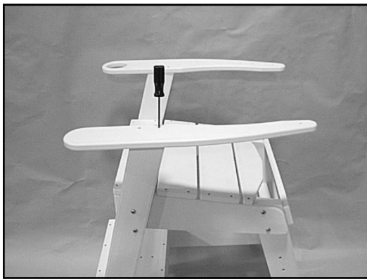
7. Attach right and left arm rests to front legs using four 2" screws (right arm rest has hole for cup holder).
